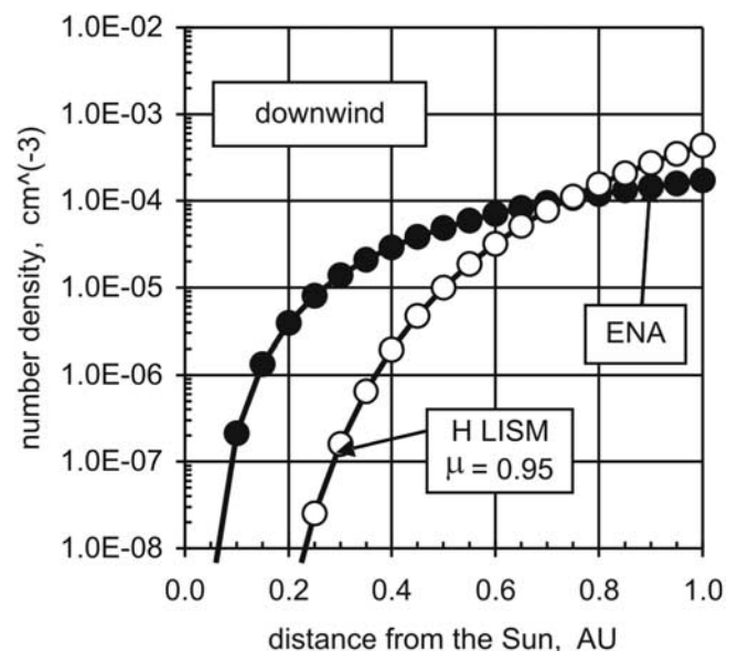
Figure 4. Radial dependence of number densities of interstellar atomic hydrogen and heliospheric ENAs for the downwind direction.
